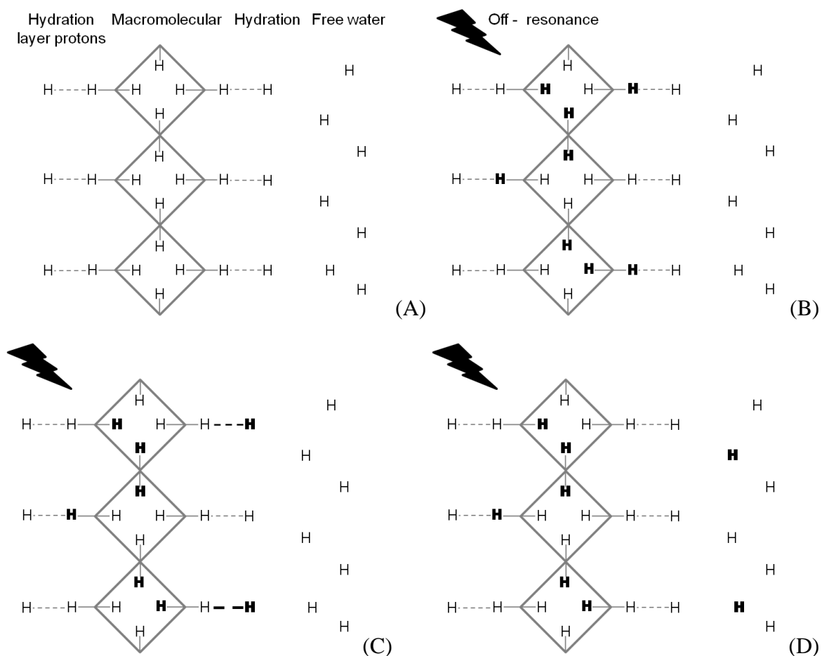
Figure 2.22. Exchange of longitudinal magnetization. Off-resonance RF pulse (black arrows) saturates the restricted macromolecular protons (unsaturated protons are designated H , while saturated are designated H )
